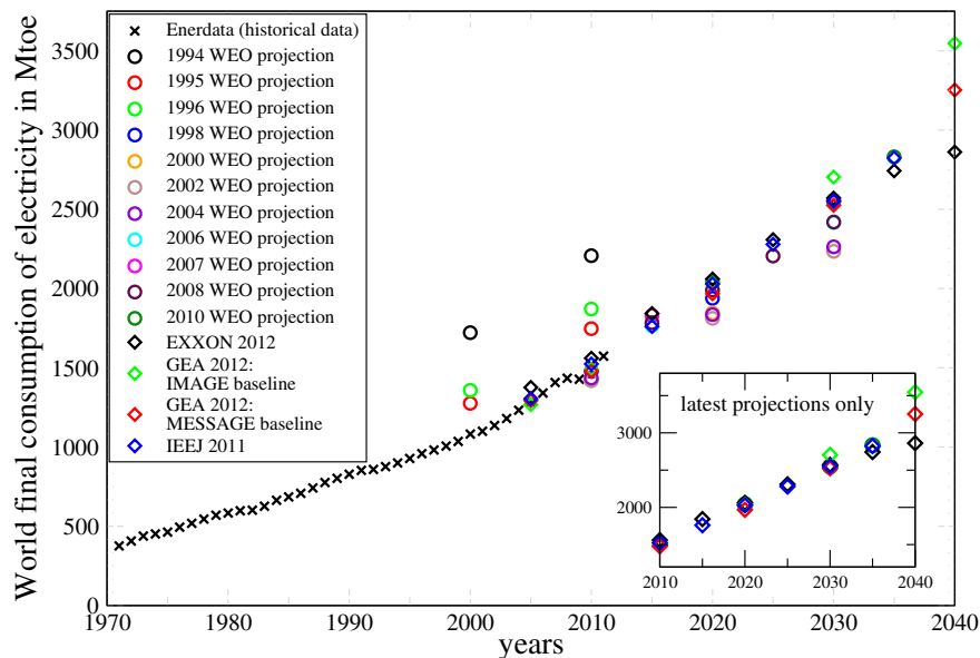
Fig. 3. Projections of world electricity demand by WEO (1994–2010), Exxon Mobil (2012), Institute of Electrical Engineers Japan (2011), and GEA (2012). Historical data are from ENERDATA. Projections show an over-estimation of electricity demand in the 90s. The spread across projections increases the further the models look into the future.
